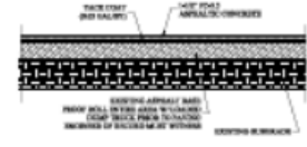
ASPHALT PAVING DETAIL
